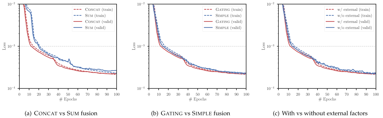
Fig. 7. Training curves on TaxiNYC of various fusions. The vertical axis corresponds to training and validation (valid) losses, and the horizontal axis corresponds to the number of epochs.
